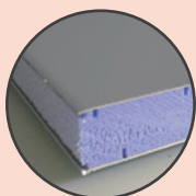
Panneau sandwich R = 0.39 \text{ m}^2\cdot\text{K}/\text{W}
